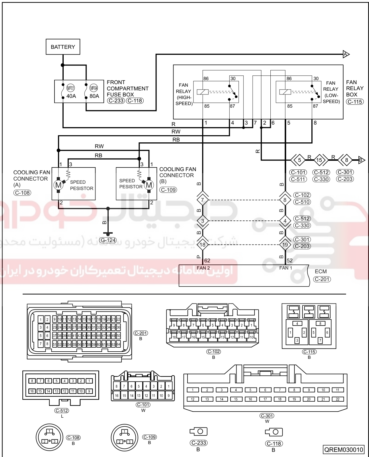
Engine circuit diagram (page 1)
