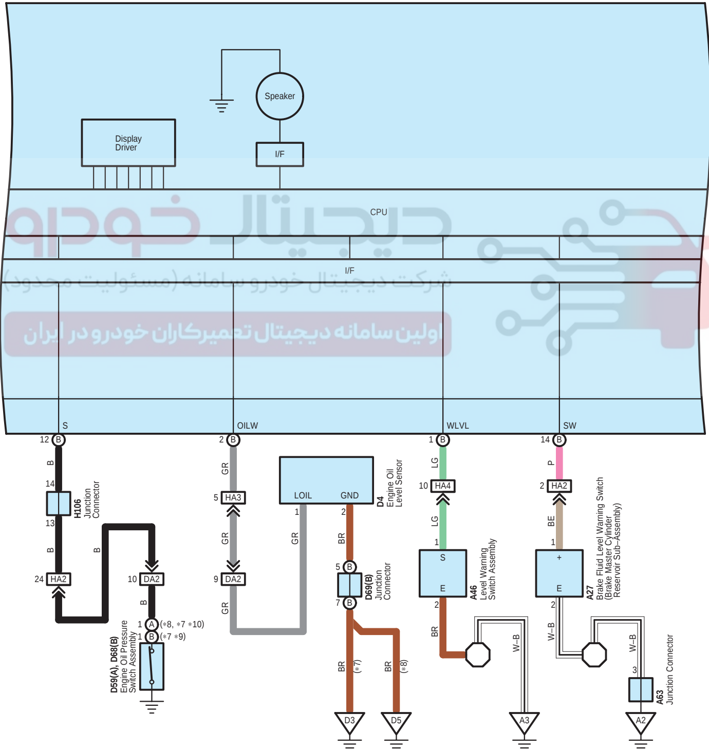
H13(A), H14(B) Combination Meter Assembly
