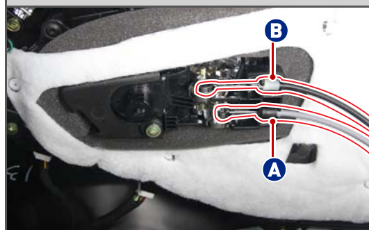
Inside handle cable (A) & Front door safety knob cable (B)
