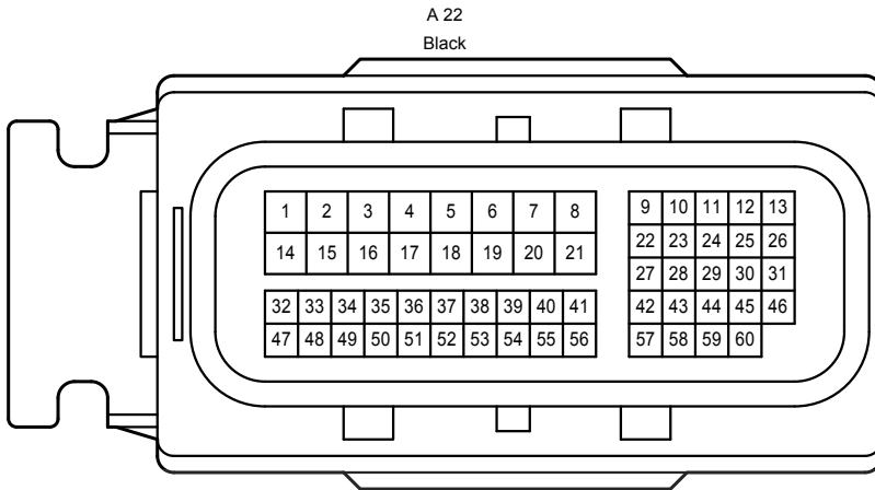
(High, Front Side Marker Light and Headlight Leveling Motor)
