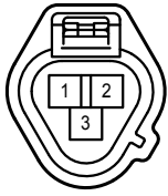
(Front Turn Signal Light and Clearance Light)
