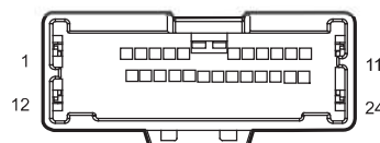
I3_MB Main W.H. Connector 3 Connecting Body W.H.
