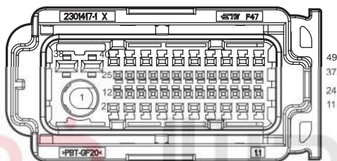
I_FLDB 左前门线束接车身线束 FL Door W.H. Connector Connecting Body W.H.
