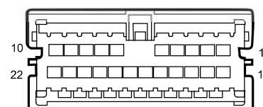
I5_MB Main W.H. Connector 5 Connecting Body W.H.
