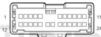
I2_MB Main W.H. Connector 2 Connecting Body W.H.
