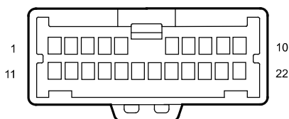
I5_BM Body W.H. Connector 5 Connecting Main W.H.
