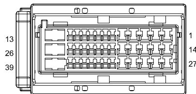
I1_ME Main Harness to Engine Harness 1
