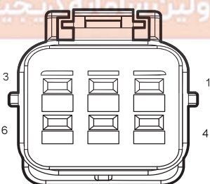
F19 Left Outer Combination Light
