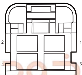
E09 Brake Pedal Switch
