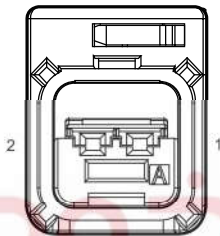
F18 Driver Airbag
