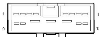
I3_BE Body W.H. Connector 3 Connecting Engine W.H.
