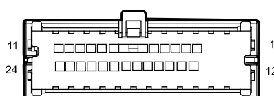
I4_MB Main W.H. Connector 4 Connecting Body W.H.
