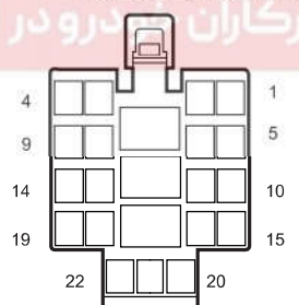
I1_EB Engine W.H. Connector 1 Connecting Body W.H.
