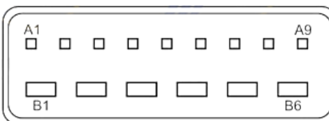
Connector 15 Pin White
