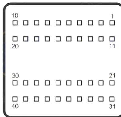
Connector 40 Pin Black
