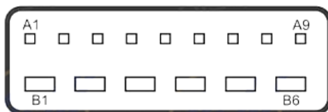
Connector 15 Pin Black
